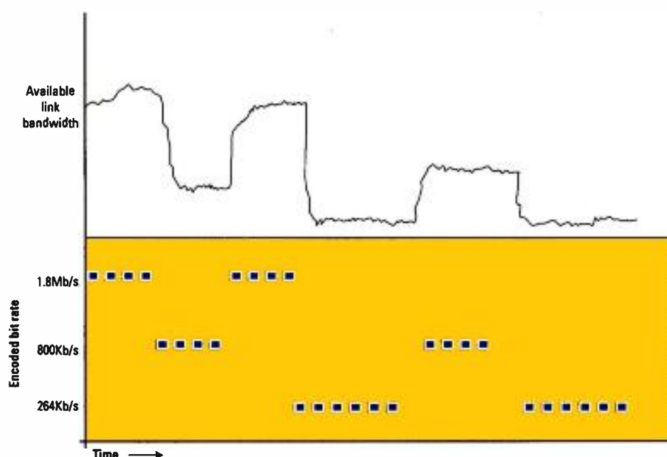
Figure 1. As available link bandwidth changes, the receiver requests content encoded at lower or higher bit rates.
