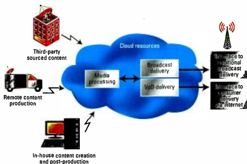
Figure 5. In this streamed media example, the cloud represents multiple servers located in different geographical regions so that the fastest and most bandwidth-efficient service can be offered to consumers worldwide.
