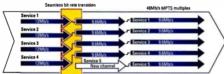
Figure 1. Example of a 48Mb/s multiplex of four services being modified to five services
