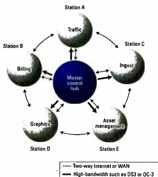
Figure 1. This hybrid centralcasting variation spreads the workflow across a group of stations.
