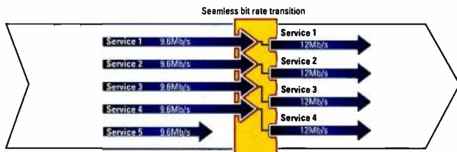
Figure 2. Example of a 48Mb/s multiplex of five services being modified to four services
