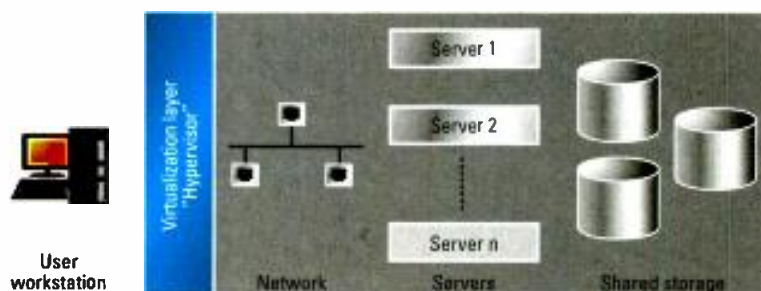
Figure 2. Using virtualization, a single server, or groups of servers, may be set up as multiple VMs. The Hypervisor abstracts the VMs from the underlying hardware (host server), allowing the creation of multiple VMs that can use the available hardware resources.
